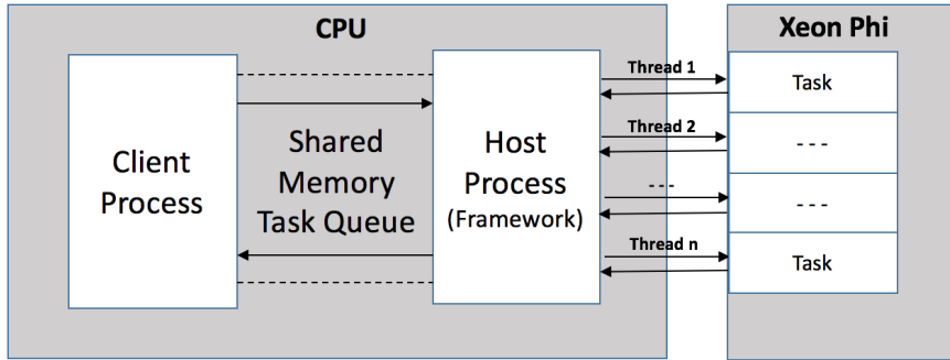
Fig. 3.2: OpenMP-Phi diagram.
