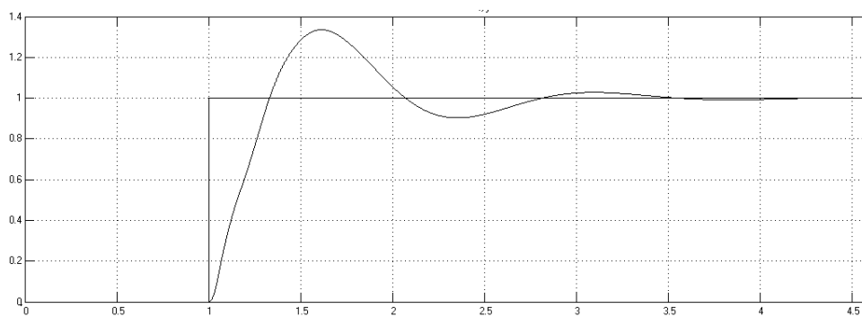
FIG. 6.6. System response.
