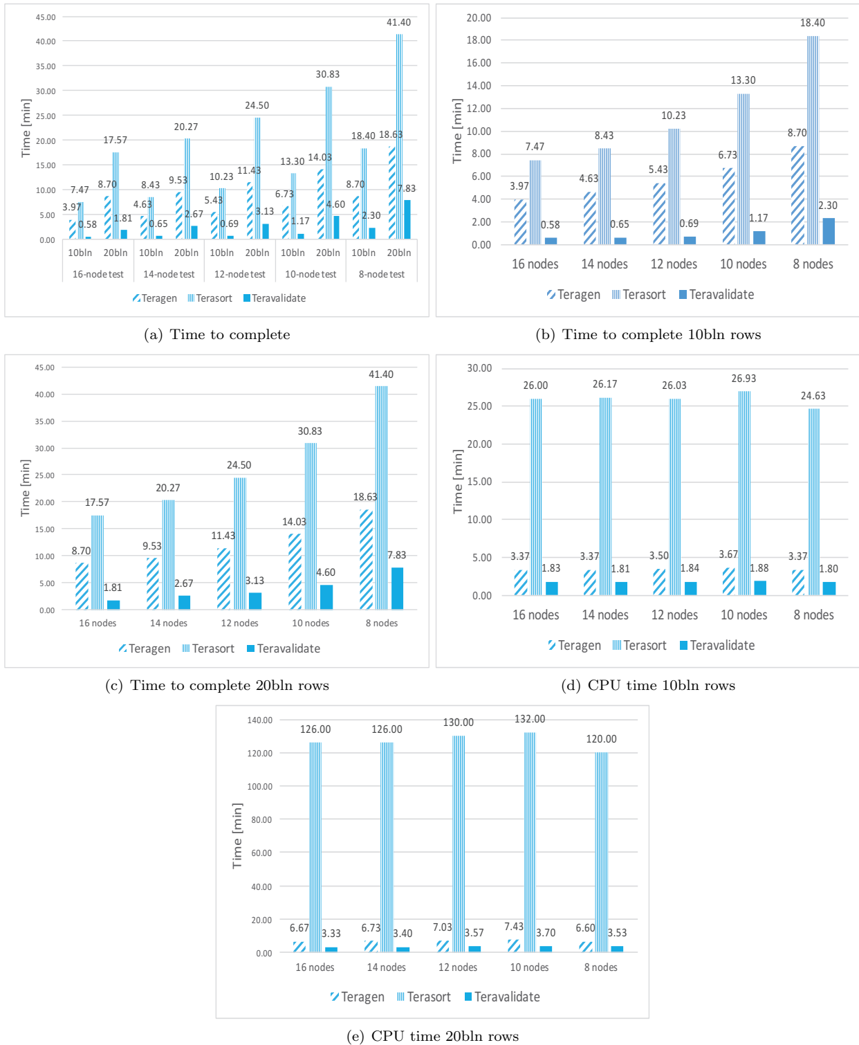
Fig. 5.2: Time to complete and CPU time for 16, 14, 12, 10 and 8 nodes
